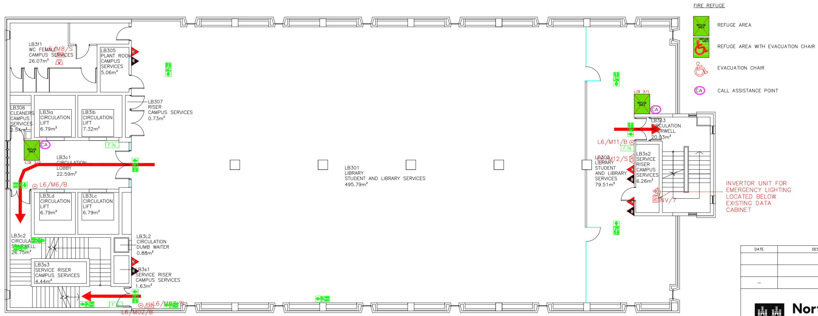
LIBRARY BUILDING THIRD FLOOR PLAN 742.03m 2
